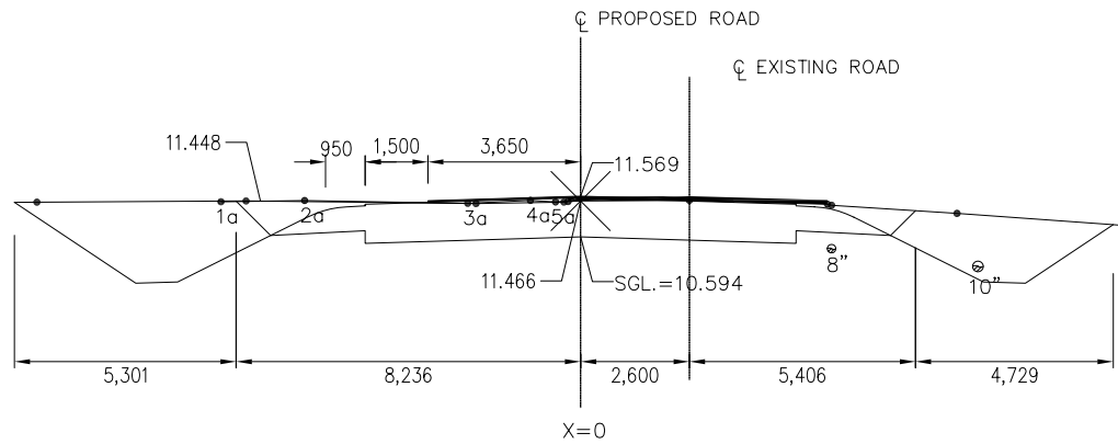
CROSS SEC. AT Ch. 1+880
