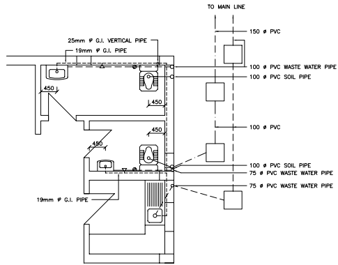
DETAIL PLAN (GROUND & FIRST FLOOR) SCALE 1:50
