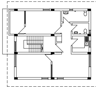
FIRST FLOOR PLAN SCALE 1:100
