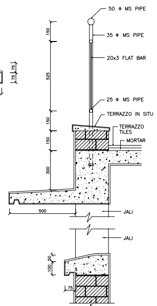
DETAIL SCALE 1:10 ⑪
