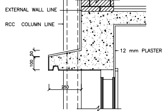
DETAIL SCALE 1:10 ⑧
