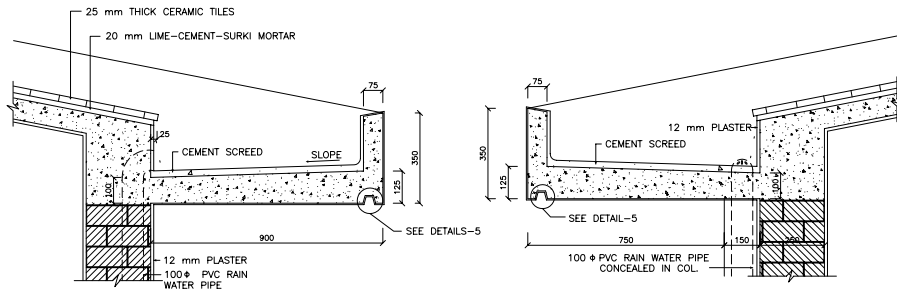
DETAIL SCALE 1:10 ⑦
