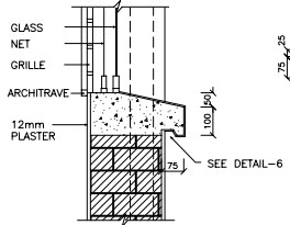
DETAIL SCALE 1:10 ③
