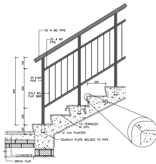
TYPICAL STAIR RAILING DETAIL SCALE 1:10
