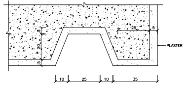
DETAIL SCALE 1:1 ⑤
