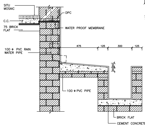
DETAIL SCALE 1:10 ④
