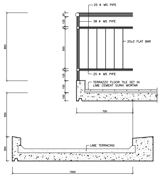
DETAIL SCALE 1:10 ⑨
