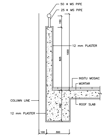
DETAIL SCALE 1:10 ⑩
