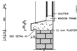
DETAIL SCALE 1:10 ⑫
