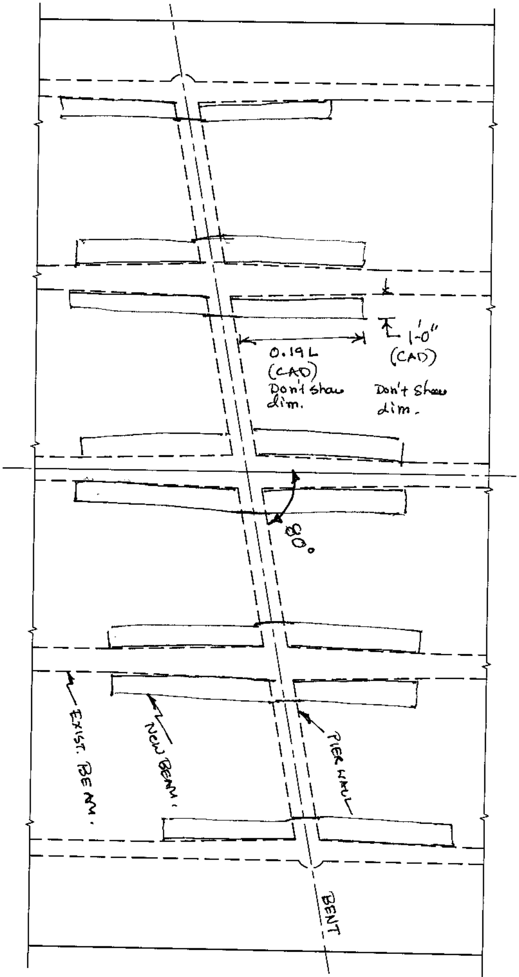
PLAN OF CAP Scale: 1/4" = 1'-0"
