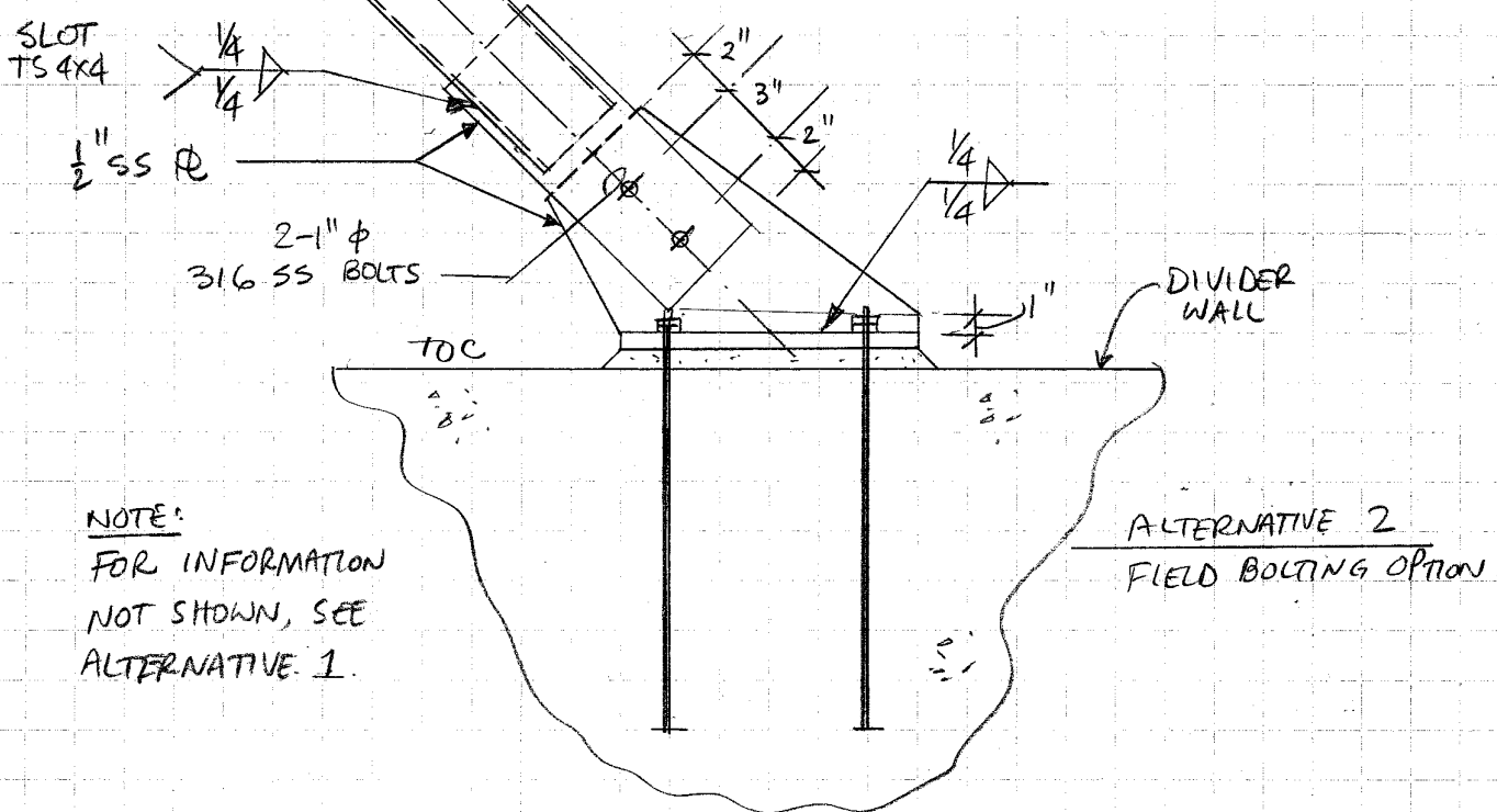
ALTERNATIVE 1 FIELD WELDING OPTION
