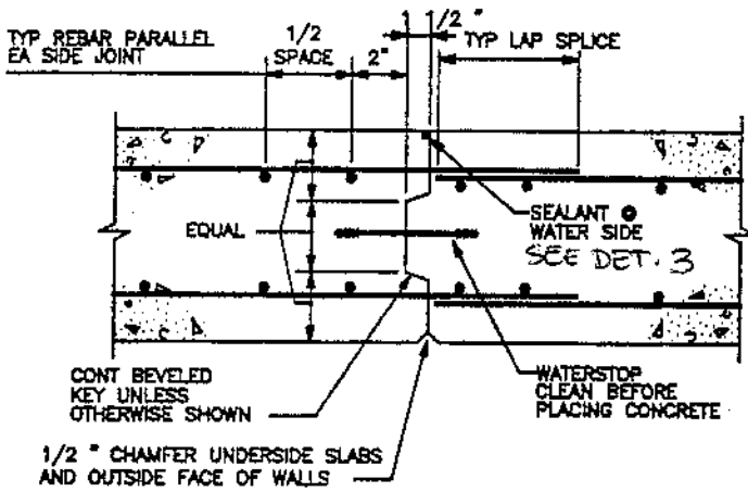
WATER BEARING WALL, FLOOR AND ROOF SLABS
