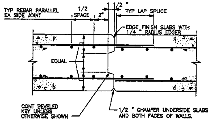
NON-WATER BEARING WALL OR SLAB
