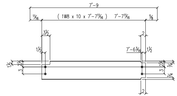
1 - BEAM - 153B2
