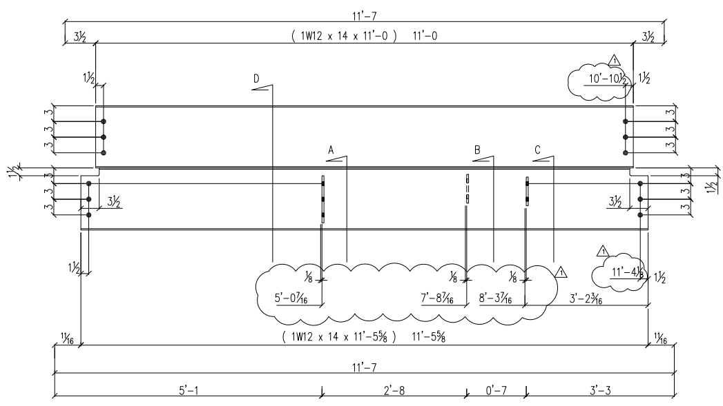
1 - BEAM - 153B3
