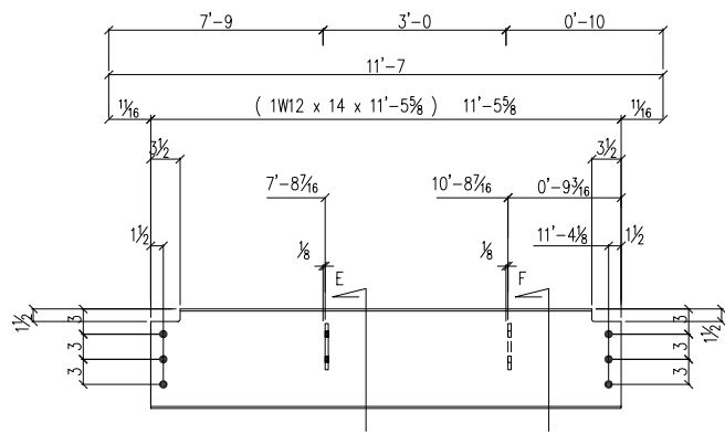
1 - BEAM - 153B1
