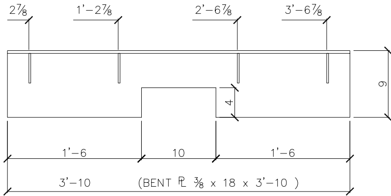
SECT-"B - B"
