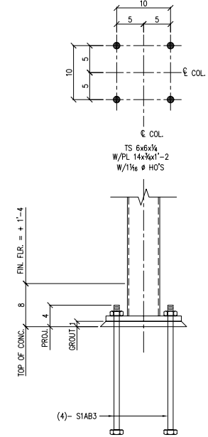
COL. BASE DETAIL # 2a (2 PLACES)
