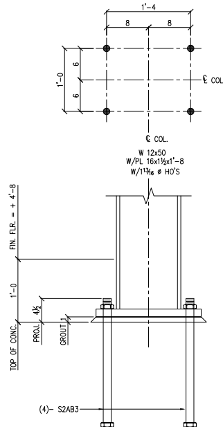
COL. BASE DETAIL # 4 (1 PLACE)
