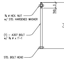
214 - ANCHOR BOLT - S1AB3
