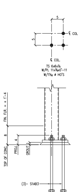
COL. BASE DETAIL # 3 (1 PLACE)
