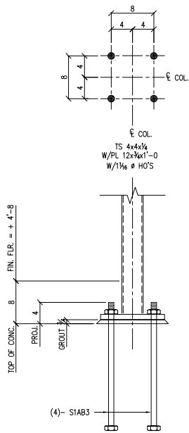
COL. BASE DETAIL # 1 (38 PLACES)
