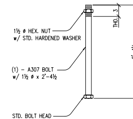
4 - ANCHOR BOLT - S2AB3
