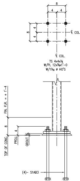
COL. BASE DETAIL # 1b (1 PLACE)
