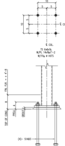
COL. BASE DETAIL # 2 (6 PLACES)
