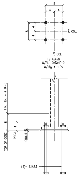
COL. BASE DETAIL # 1a (4 PLACES)
