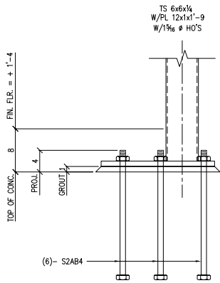
COL. BASE DETAIL # 8a ( 1 PLACE )
