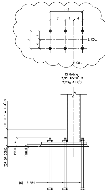
COL. BASE DETAIL # 7 ( 2 PLACES )
