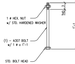
12 - ANCHOR BOLT - S2AB4
