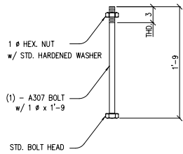
24 - ANCHOR BOLT - S1AB4
