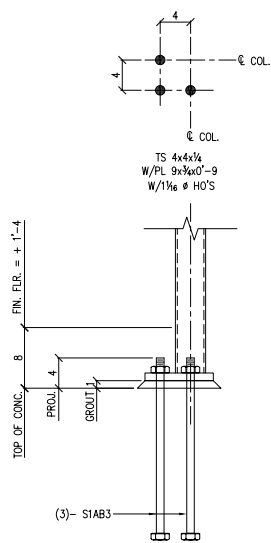
COL. BASE DETAIL # 5 ( 1 PLACE )
