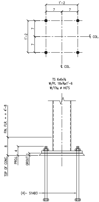
COL. BASE DETAIL # 6 ( 1 PLACE )
