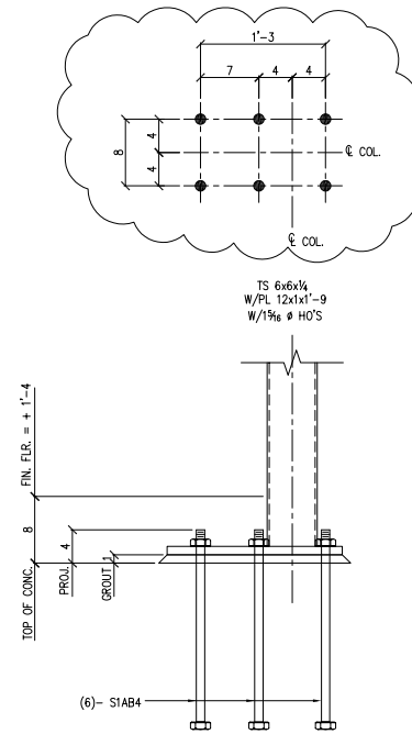
COL. BASE DETAIL # 7a ( 2 PLACES )
