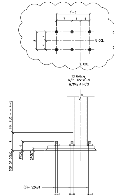
COL. BASE DETAIL # 8 ( 1 PLACE )
