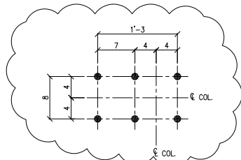
COL. BASE DETAIL # 5 ( 1 PLACE )
