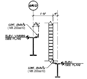
07 SECTION E4 3/4" = 1'-0" (REF. 22/54.1)
