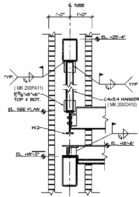
01 SECTION E4 3/4" = 1'-0" (REF. 14/54.1)
