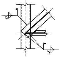
02 SECTION E4 3/4" = 1'-0" (REF. 14/54.1)
