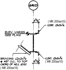
08 SECTION E4 3/4" = 1'-0" (REF. 23/54.1)
