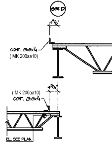
05 SECTION E4 3/4" = 1'-0" (REF. 20/54.1)
