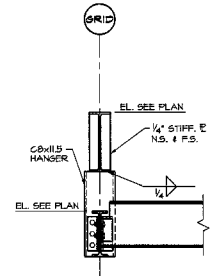
12 SECTION E4 3/4" = 1'-0" (REF. 27/54.1)
