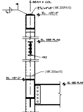
03 SECTION E4 3/4" = 1'-0" (REF. 18/54.1)
