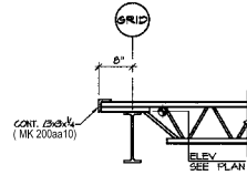
04 SECTION E4 3/4" = 1'-0" (REF. 19/54.1)
