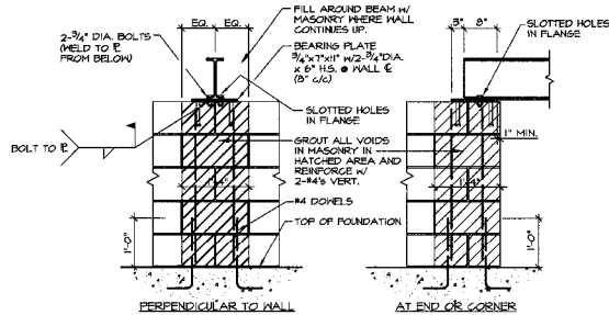
09 TYP. BEAM BRG. ON MASONRY WALL E4 N. T. S. (REF. 24/54.1)
