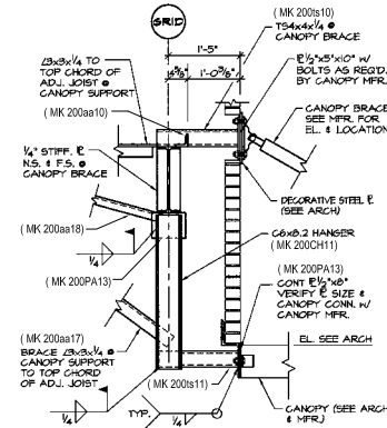
11 SECTION E4 3/4" = 1'-0" (REF. 26/54.1)
