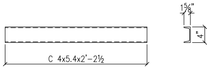
1 - CHANNEL HANGER -200CH10
