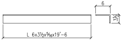
1 - ANGLE -200aa11
